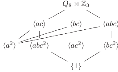
FIGURE 17. K_{3,3} in the Lattice of Q_8 \rtimes \mathbb{Z}_3
